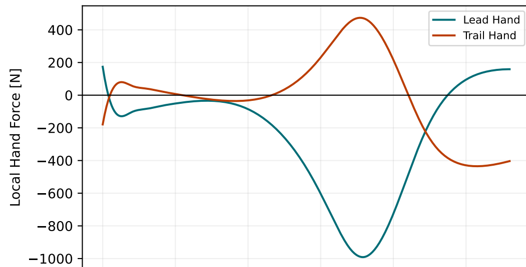
BASE — Axial
