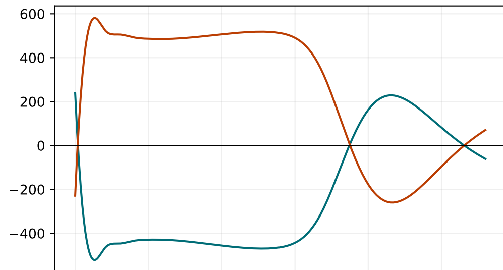
BASE — Normal
