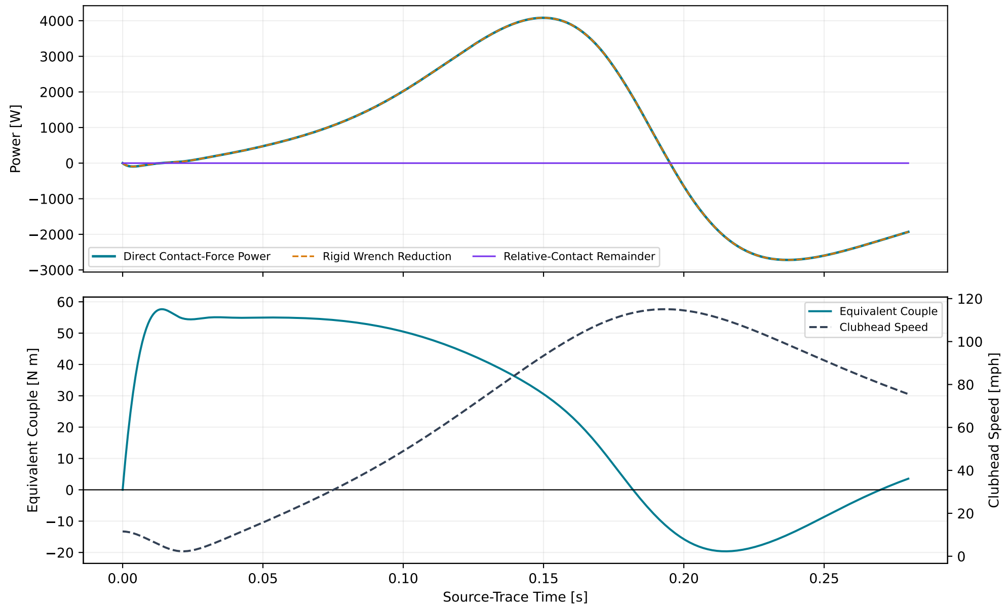
Negative Couple Sign Does Not Alone Determine Energy-Transfer Sign
