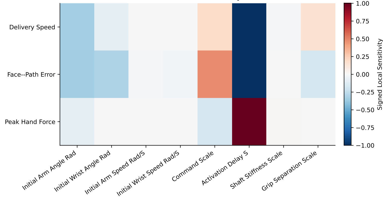
Row-Normalized Local Outcome Jacobian
