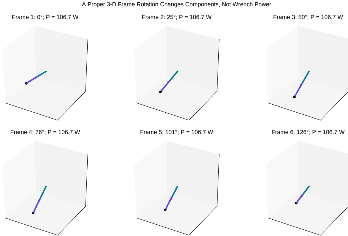
Figure 22.8: A Proper 3-D Frame Rotation Changes Components, Not Wrench Power
