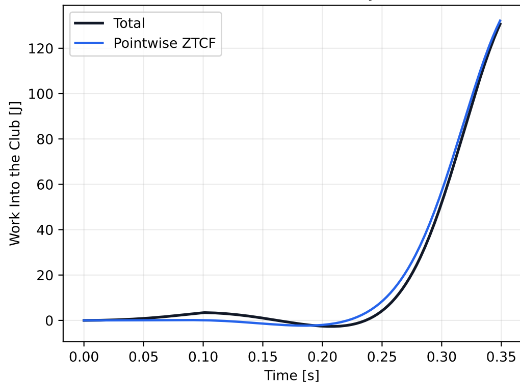
Cumulative Work Transmitted by Wrist Force
