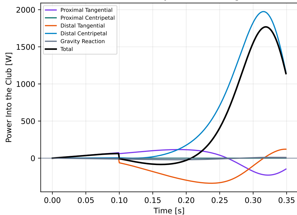
Force-Power Pathways at the Moving Wrist
