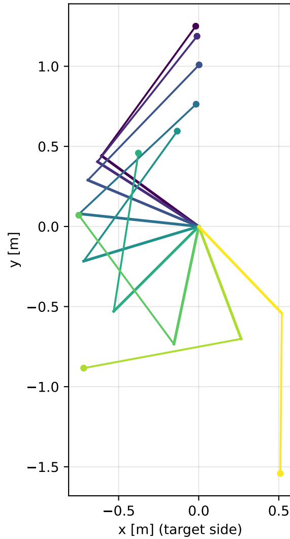
Figure 8.4: Stick-figure montage of the best restrain-then-drive swing in the swing plane (downswing progression at equal time steps).
