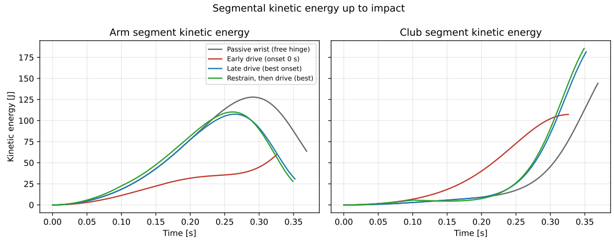
Figure 8.5: Segmental kinetic energies up to impact for the four representative programs.
