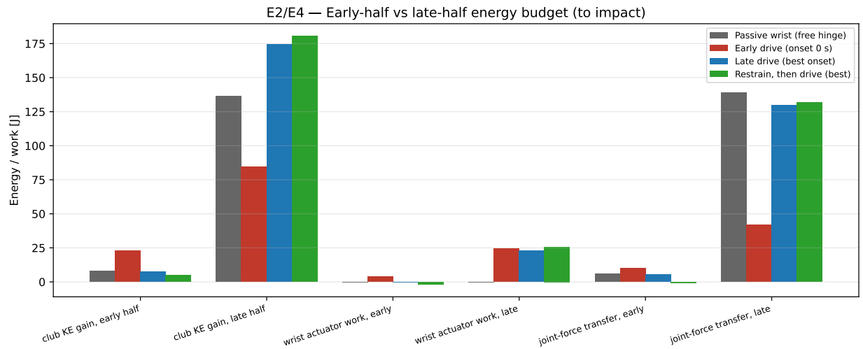
Figure 8.6: Early-half versus late-half energy budget (club kinetic-energy gain, wrist actuator work, integrated joint-force transfer) for the representative programs.
