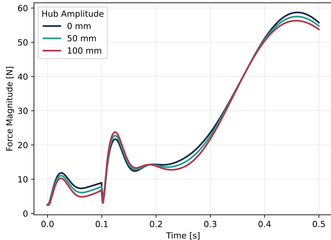
Distal Interface Force
