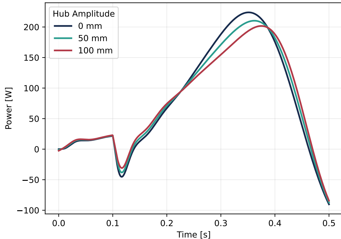
Distal Interface Wrench Power
