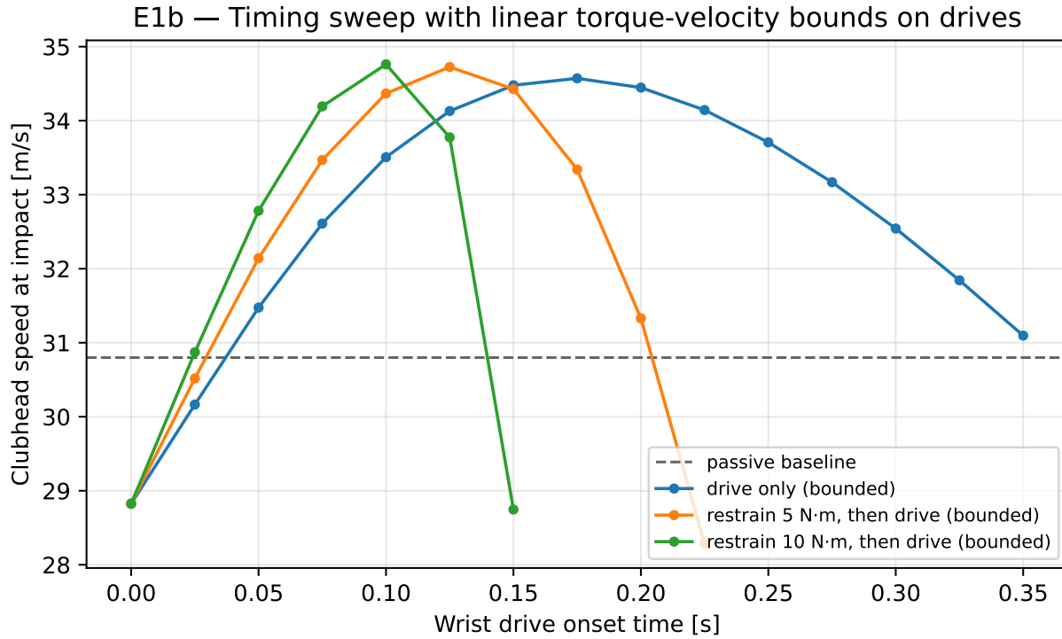
Figure 21.2: E1b: the timing sweep repeated with linear torque-velocity bounds on the shoulder and wrist drives.
