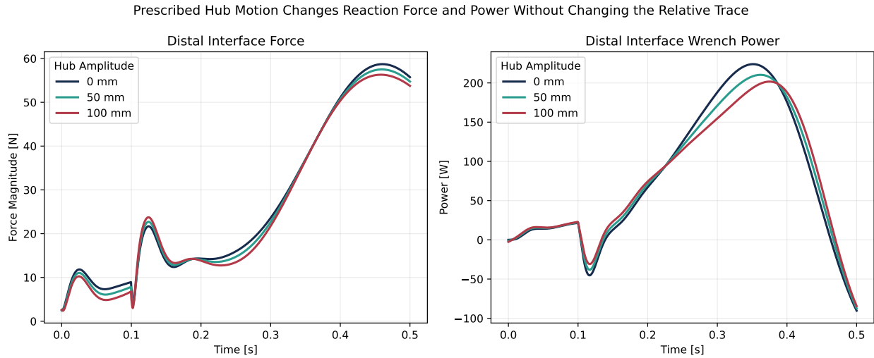
Figure 16.4: Prescribed Hub Motion Changes Reaction Force and Power Without Changing the Relative Trace
