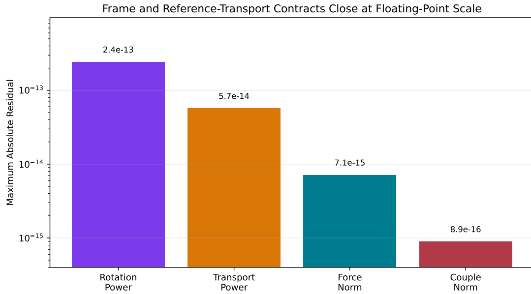
Figure 16.2: Frame and Reference-Transport Contracts Close at Floating-Point Scale
