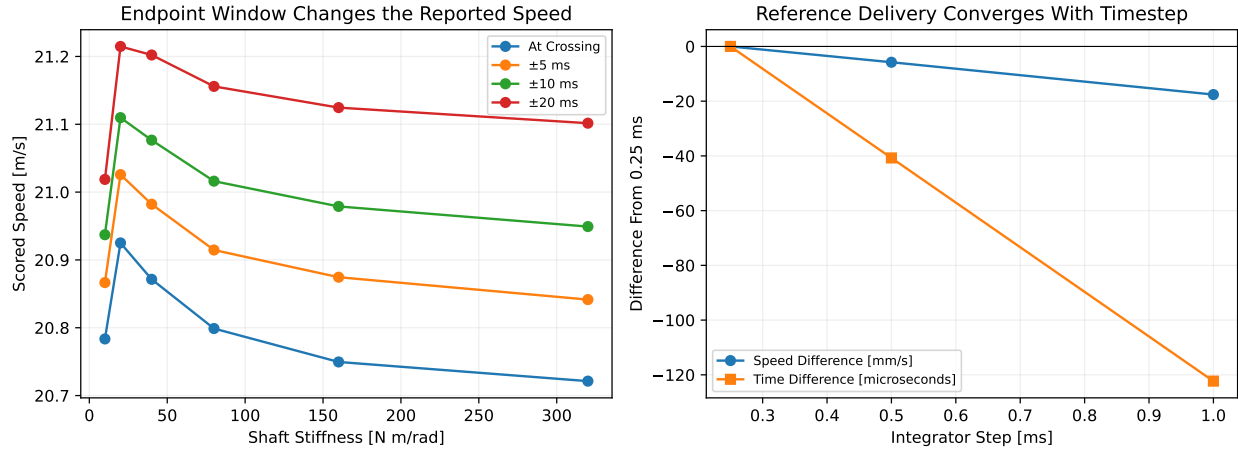
Figure 8.8: Impact Definition and Numerical Resolution
