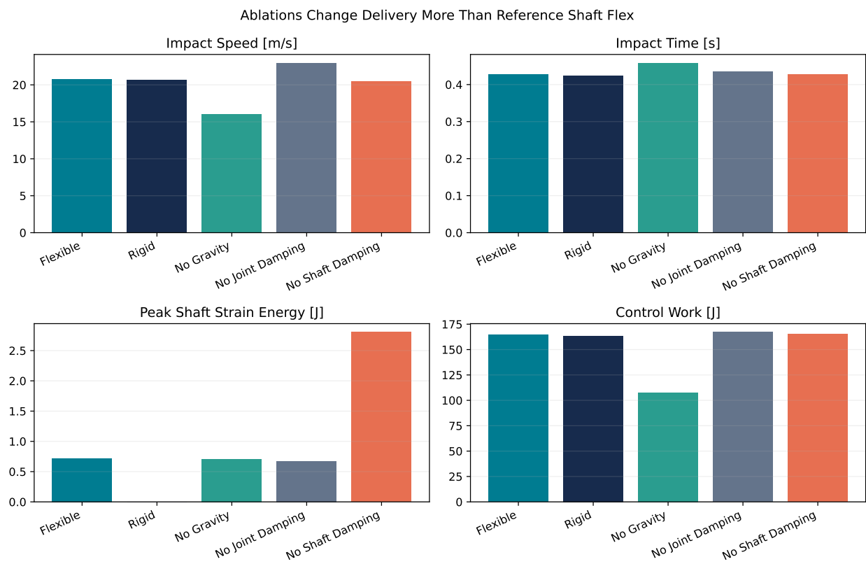
Figure 8.6: Ablations Change Delivery More Than Reference Shaft Flex
