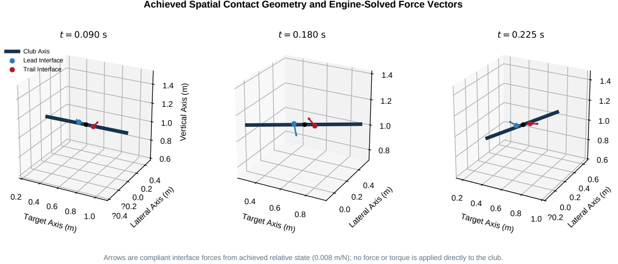
Figure 12.1: Achieved Spatial Contact Geometry and Engine-Solved Force Vectors
