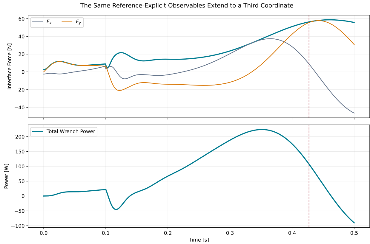
Figure 16.3: The Same Reference-Explicit Observables Extend to a Third Coordinate
