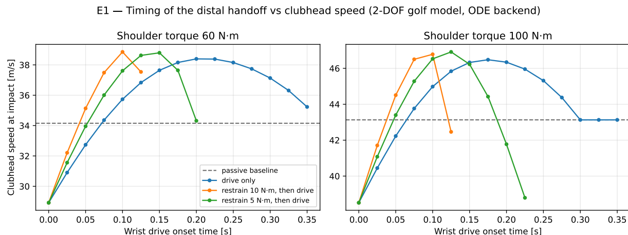
Figure 21.1: E1 sweep: clubhead speed at impact versus wrist-drive onset time, for drive-only and restrain-then-drive profiles at two shoulder-torque levels. Dashed line: fully passive wrist baseline.
