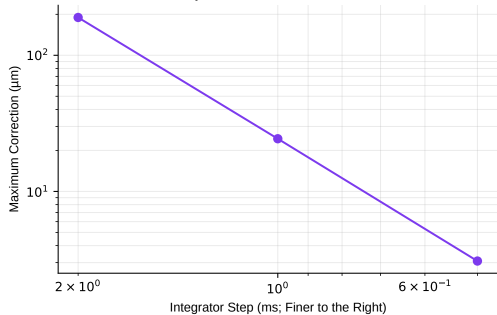
Closed-Loop Position Constraint
