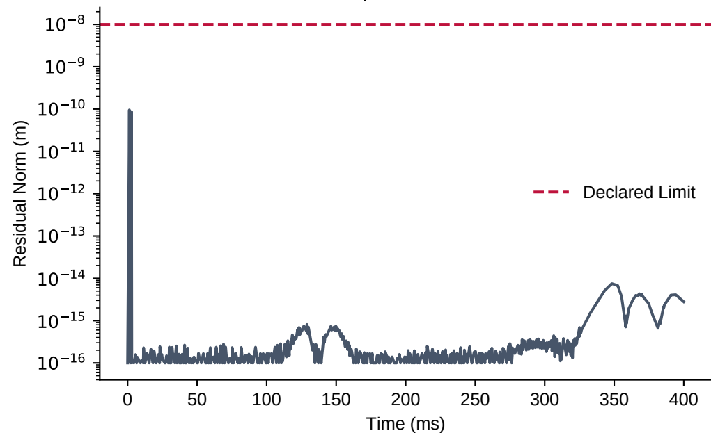
Closed-Loop Position Constraint
