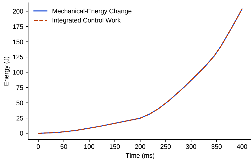
Physical Work-Energy Closure
