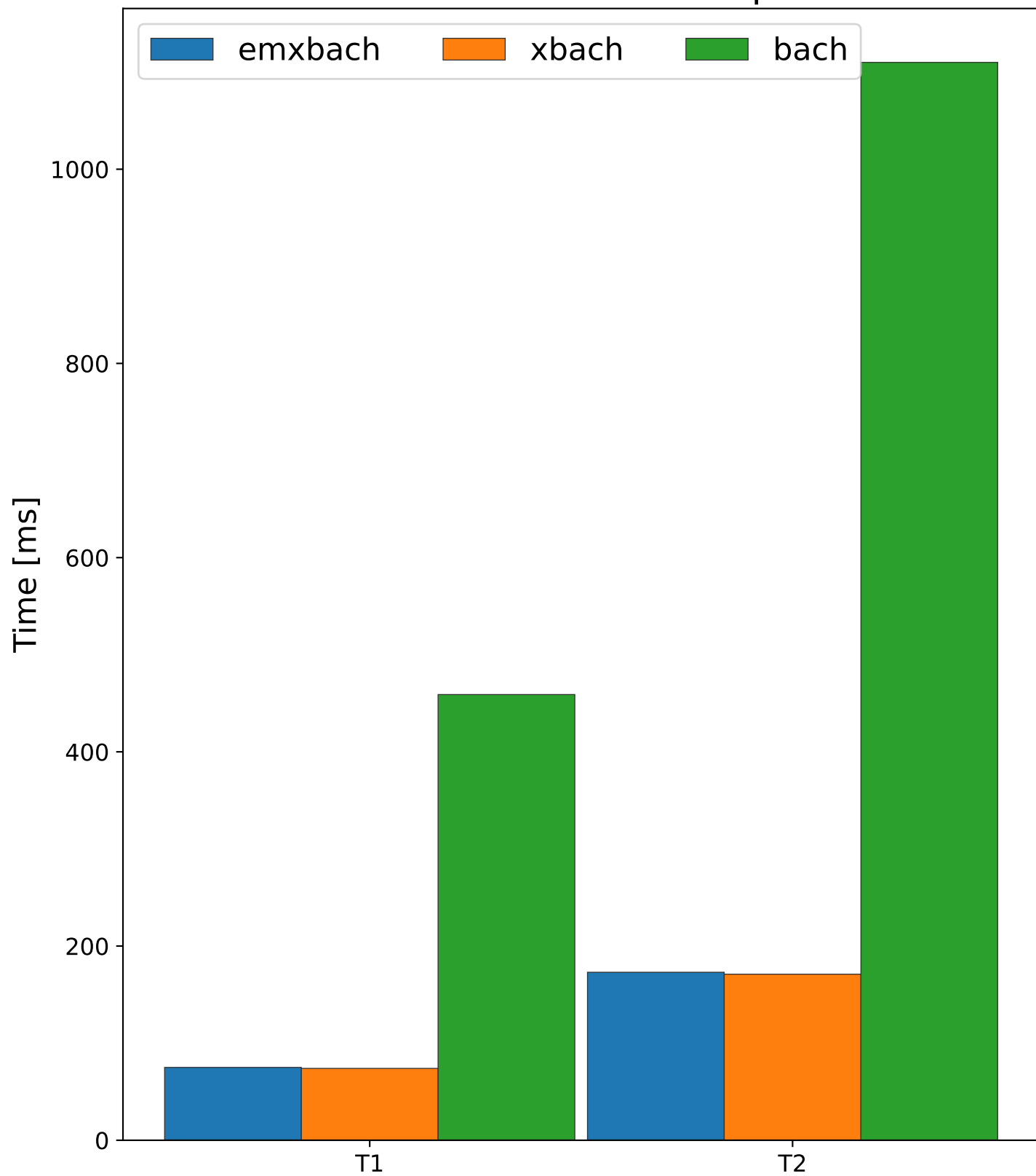
CMV execution time on computer dev
