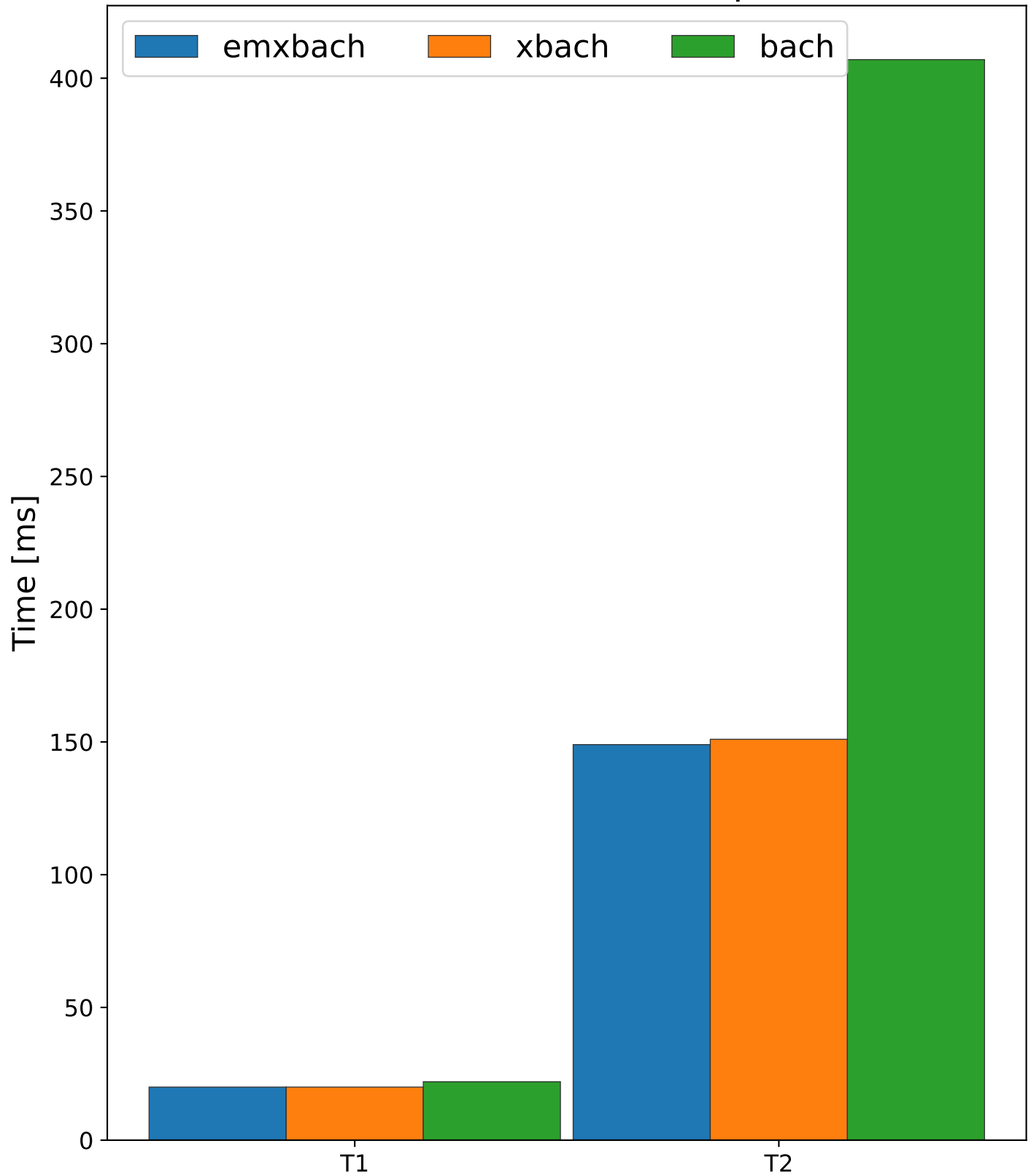
KSC execution time on computer dev
