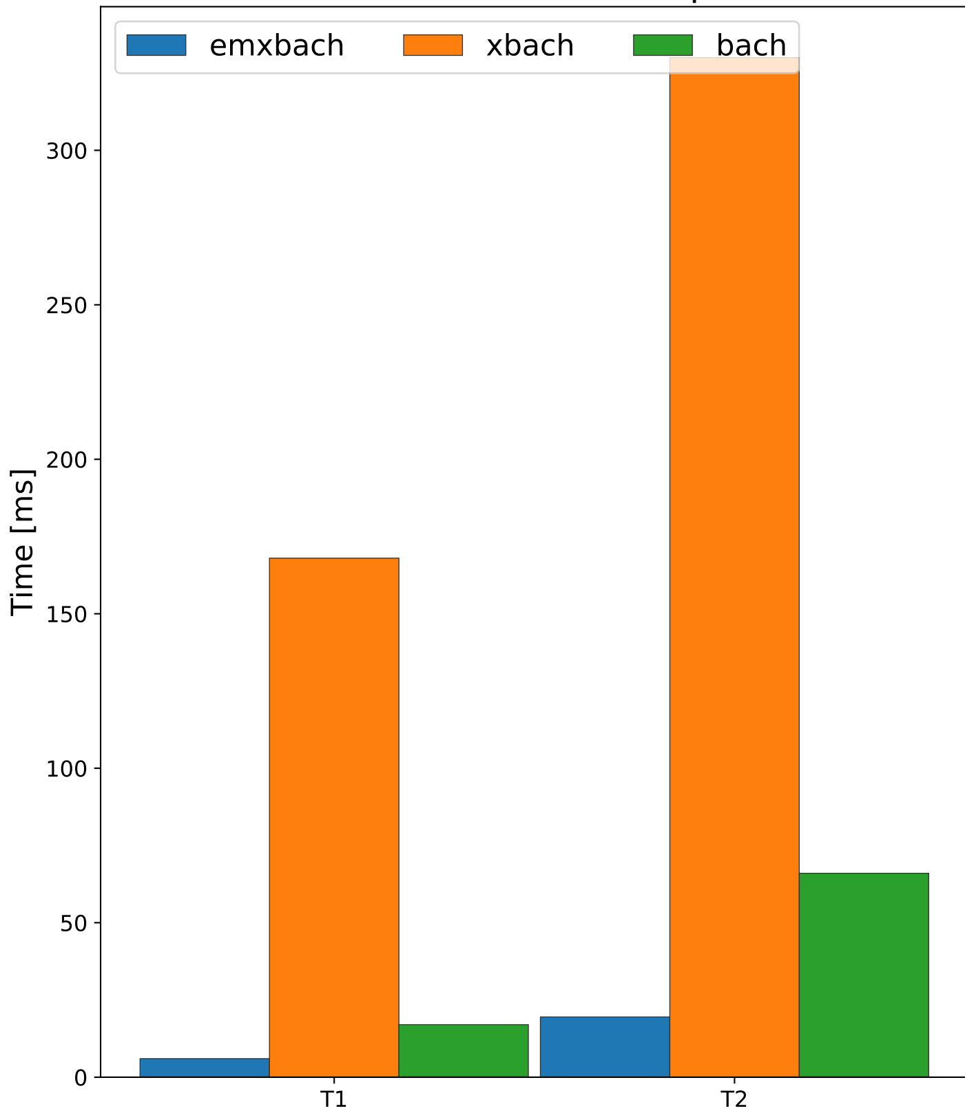
SSS execution time on computer dev
