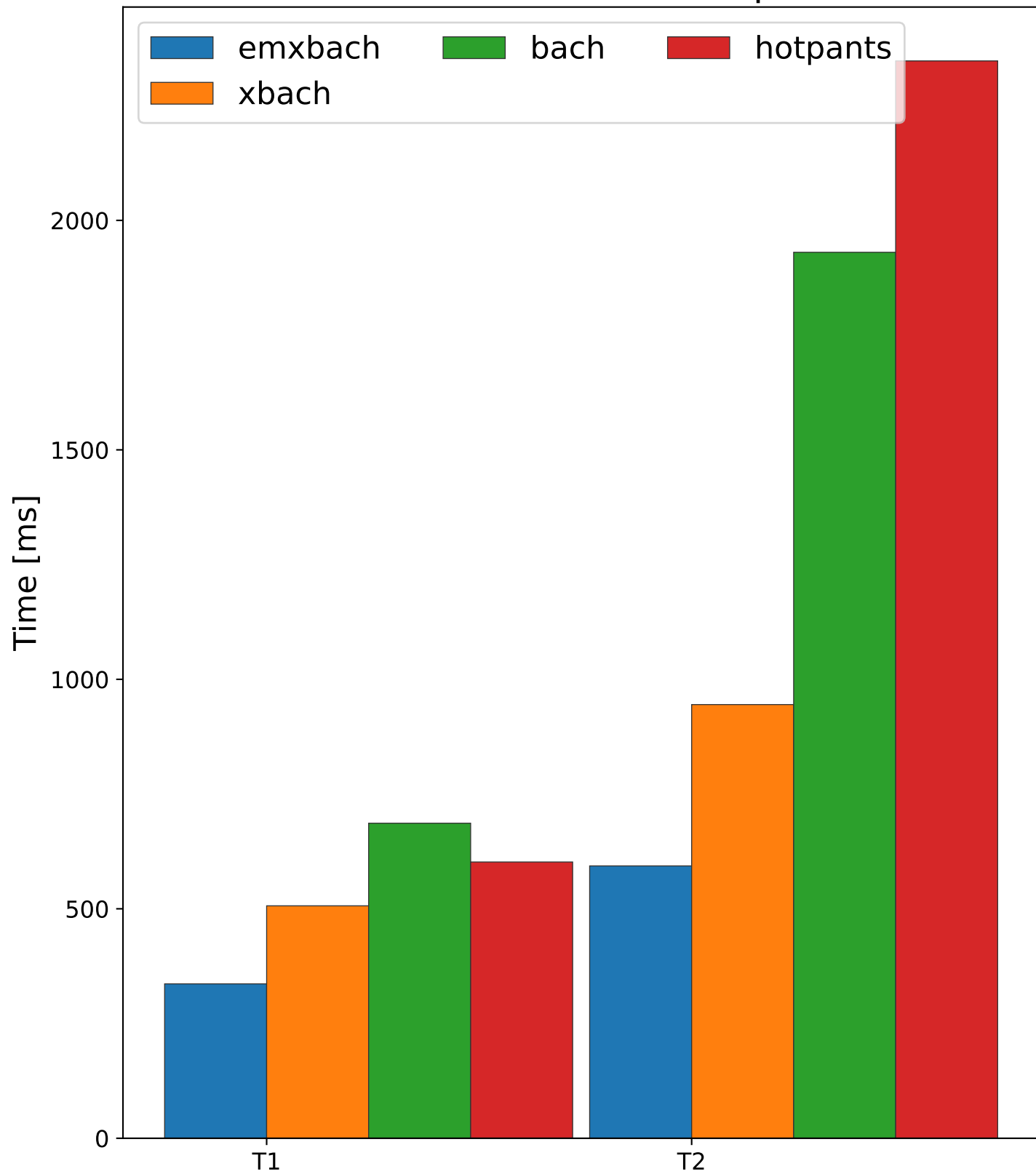
Total execution time on computer dev
