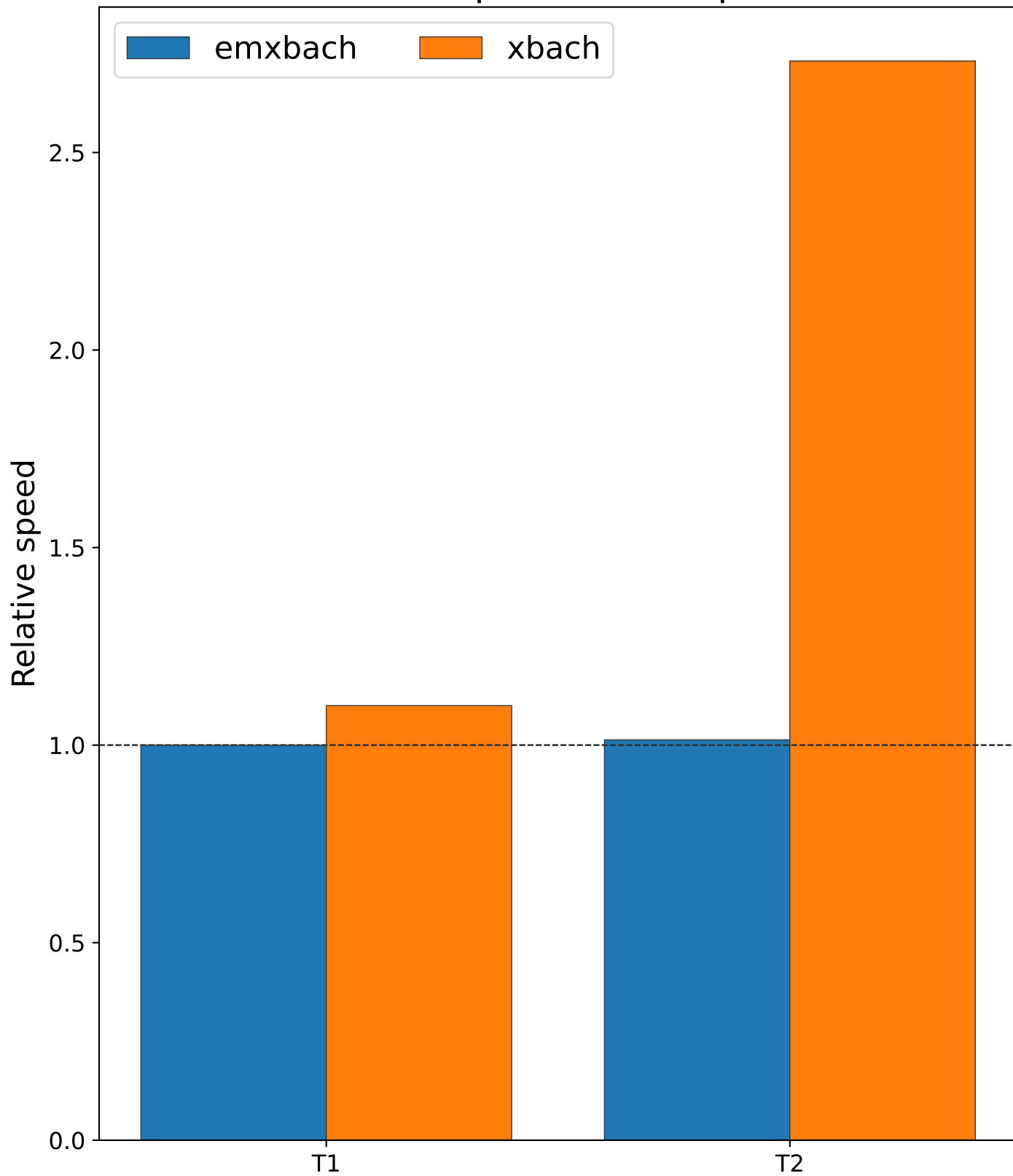
KSC relative speed on computer dev
