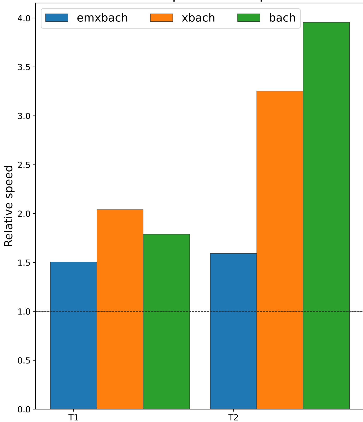
Total relative speed on computer dev
