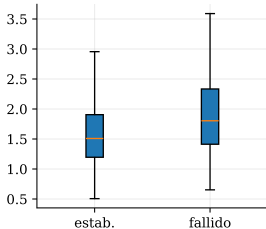
\log_{10} \kappa(A)
