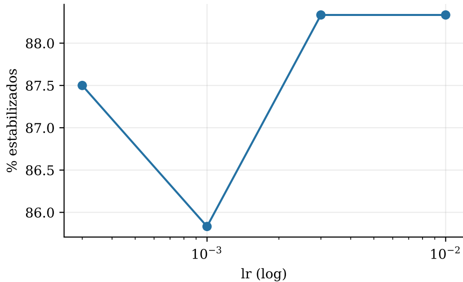
Learning rate
