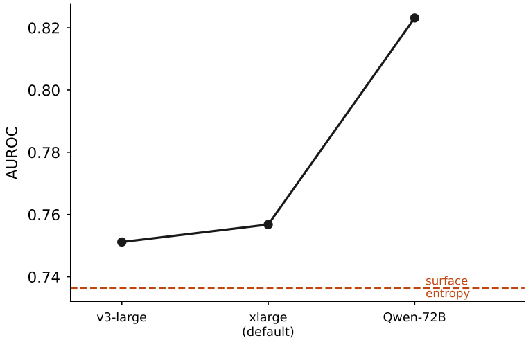
sentence-length answers
