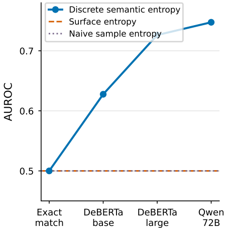
Mistral 7B
