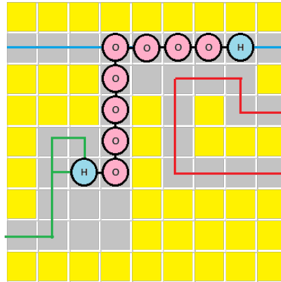
Fig. 9: Sokobond simulating a open optional door device
