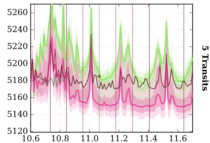
NH 3 (10.7 μm)
