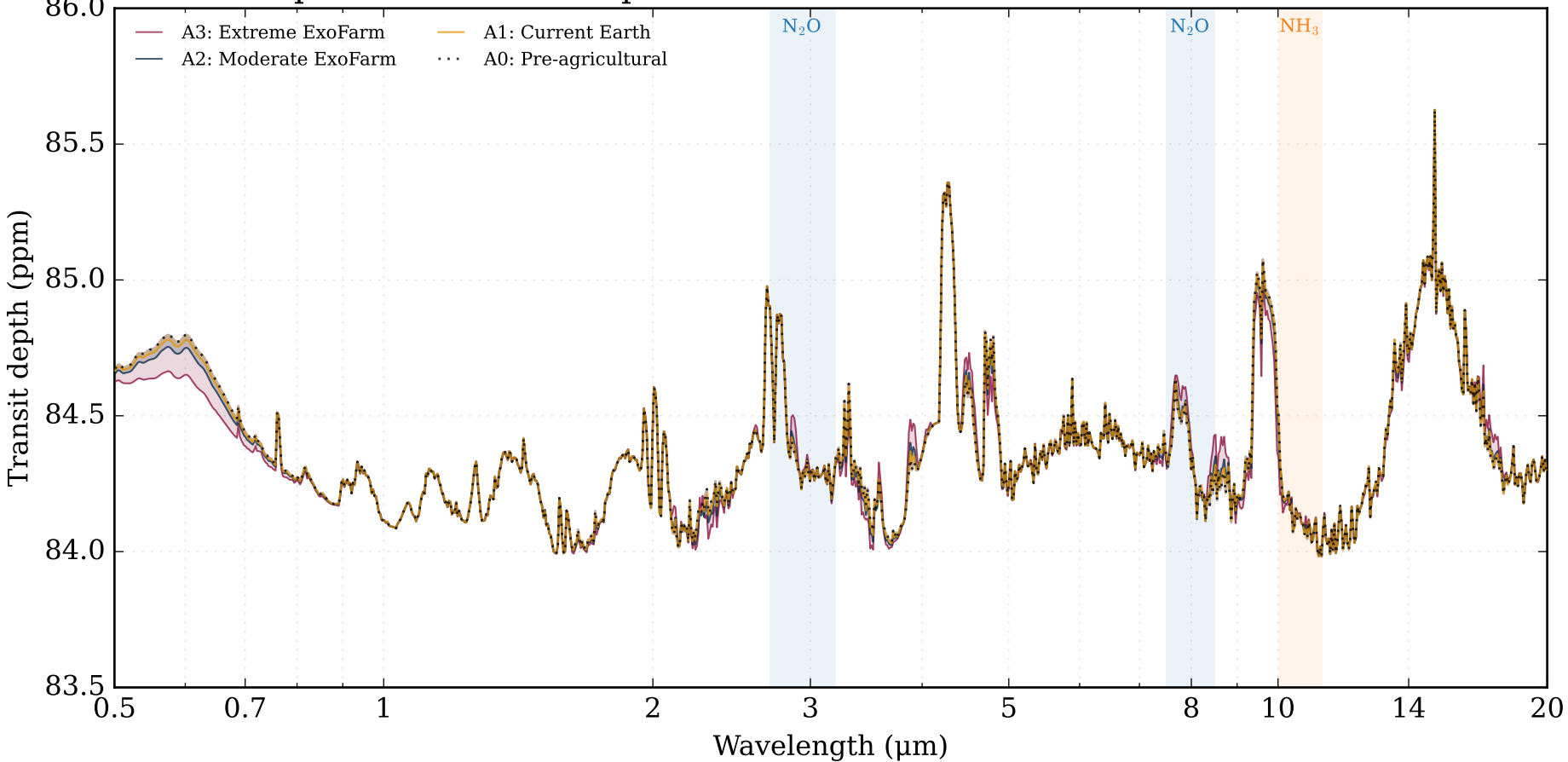
Earth-Sun pure transmission spectra
