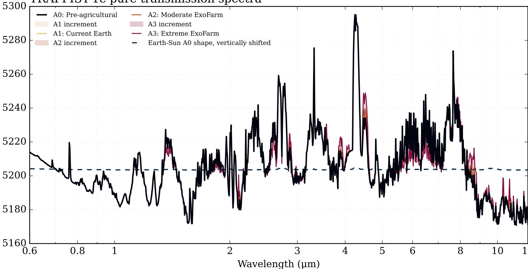
TRAPPIST-1e pure transmission spectra
