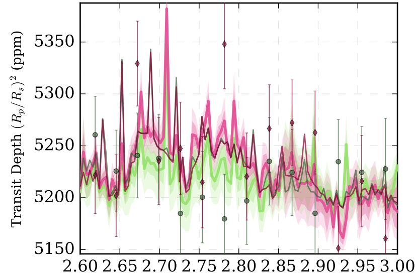
N 2 O (2.9 μm)
