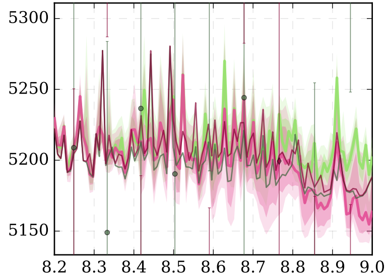
N 2 O (8.6 μm)
