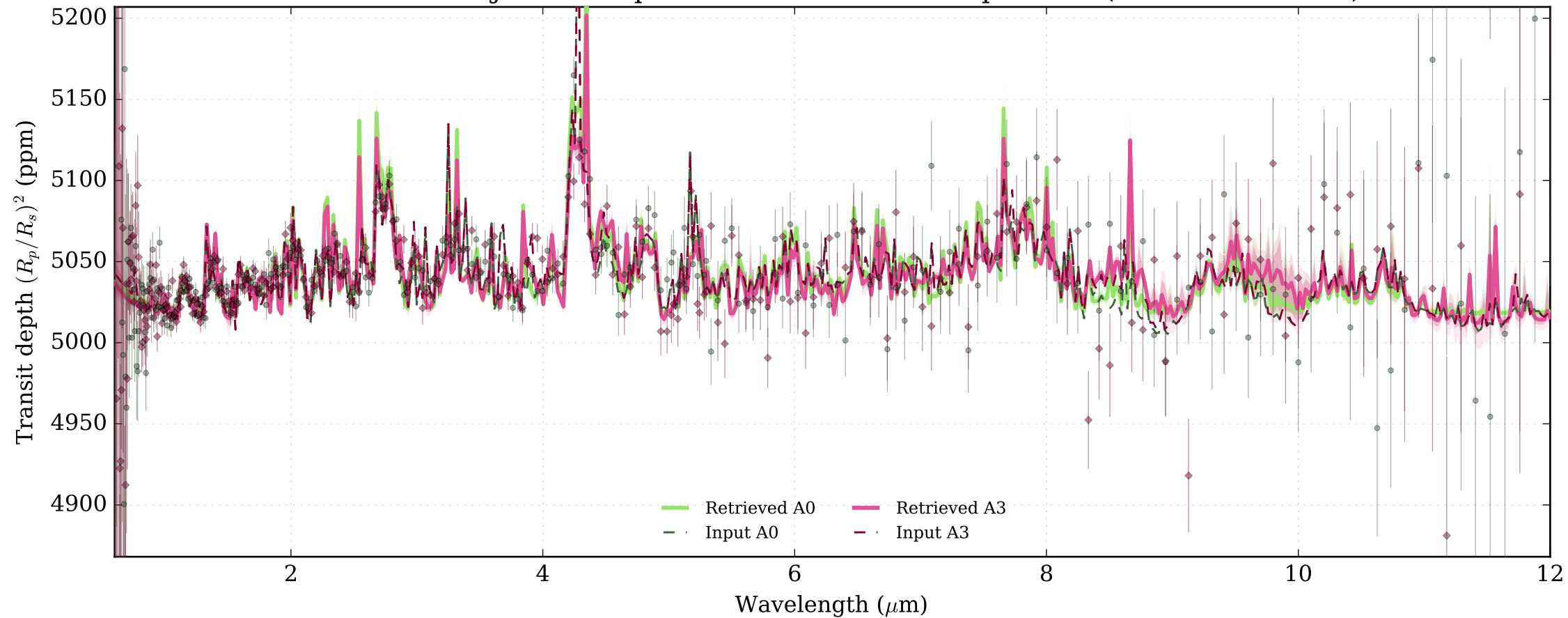
TRAPPIST-1e joint NIRSpec+MIRI retrieval: full spectrum (100+100 transits)
