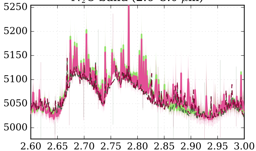
\text{N}_2\text{O} band (2.6–3.0 \mu\text{m} )
