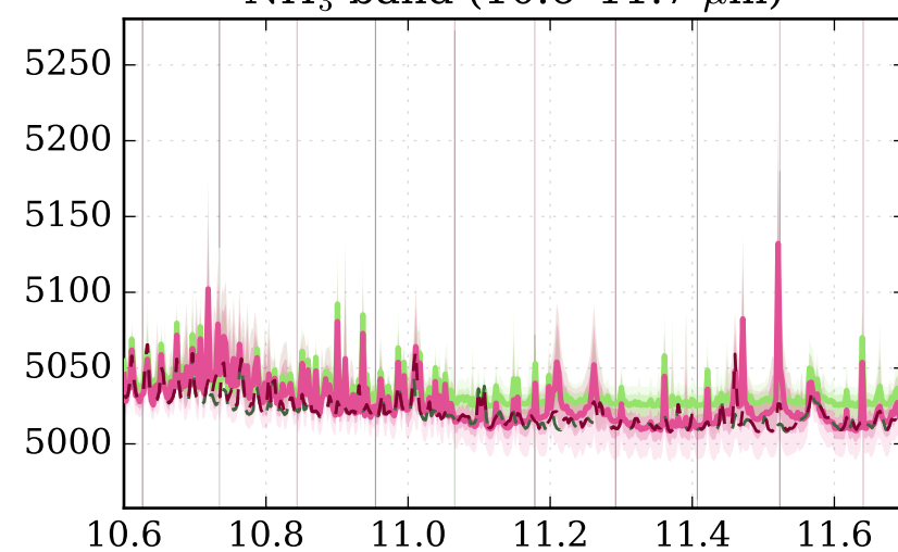
\text{NH}_3 band (10.6–11.7 \mu\text{m} )
