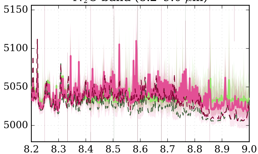
\text{N}_2\text{O} band (8.2–9.0 \mu\text{m} )
