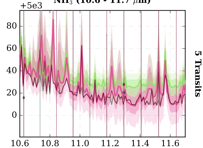
NH 3 (10.6 - 11.7 μm)
