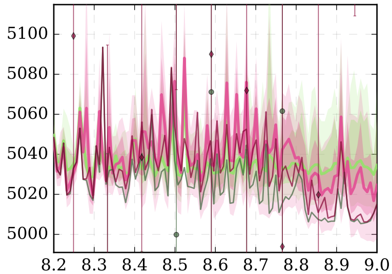
N 2 O (8.2 - 9.0 μm)
