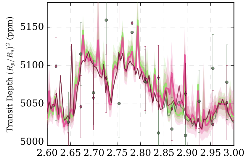
N 2 O (2.6 - 3.0 μm)
