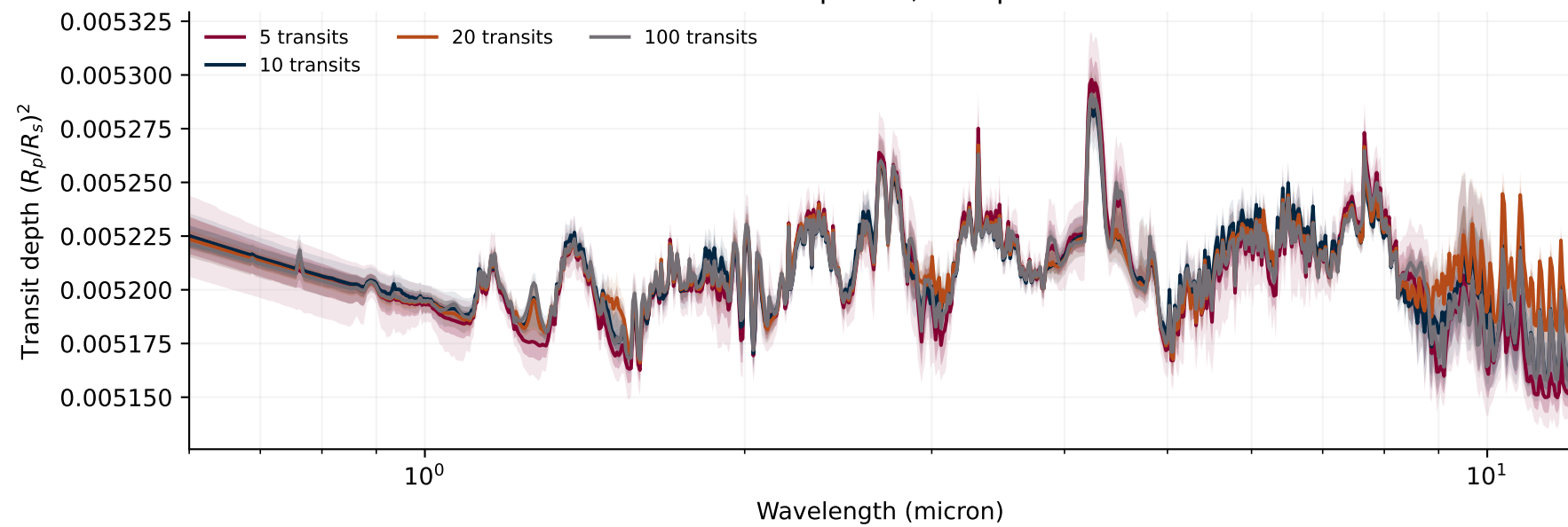
A3: retrieved spectra, NIRSpec + MIRI
