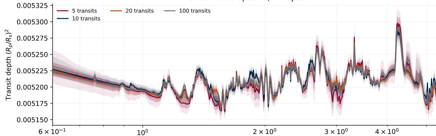
A3: retrieved spectra, NIRSpec + MIRI
