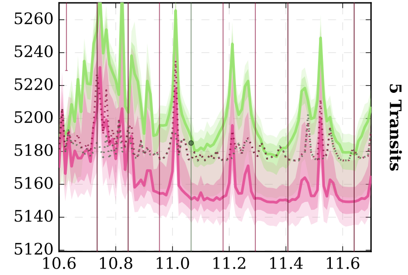
NH 3 (10.6 - 11.7 μm)
