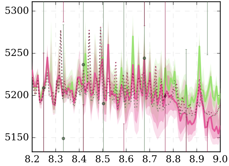
N 2 O (8.2 - 9.0 μm)
