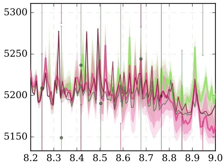
N 2 O (8.2 - 9.0 \mu\text{m} )
