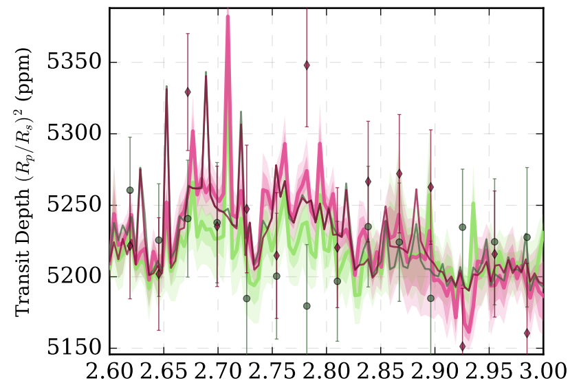
N 2 O (2.6 - 3.0 \mu\text{m} )
