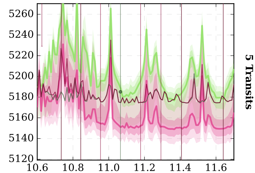
NH 3 (10.6 - 11.7 \mu\text{m} )
