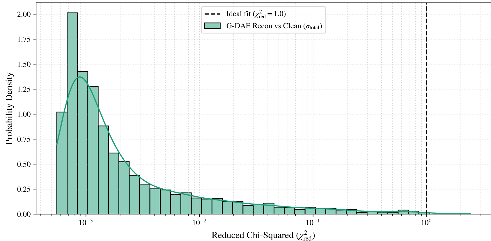
Reduced \chi^2 Distribution for Airless Transmission Spectra (10 Transits)
