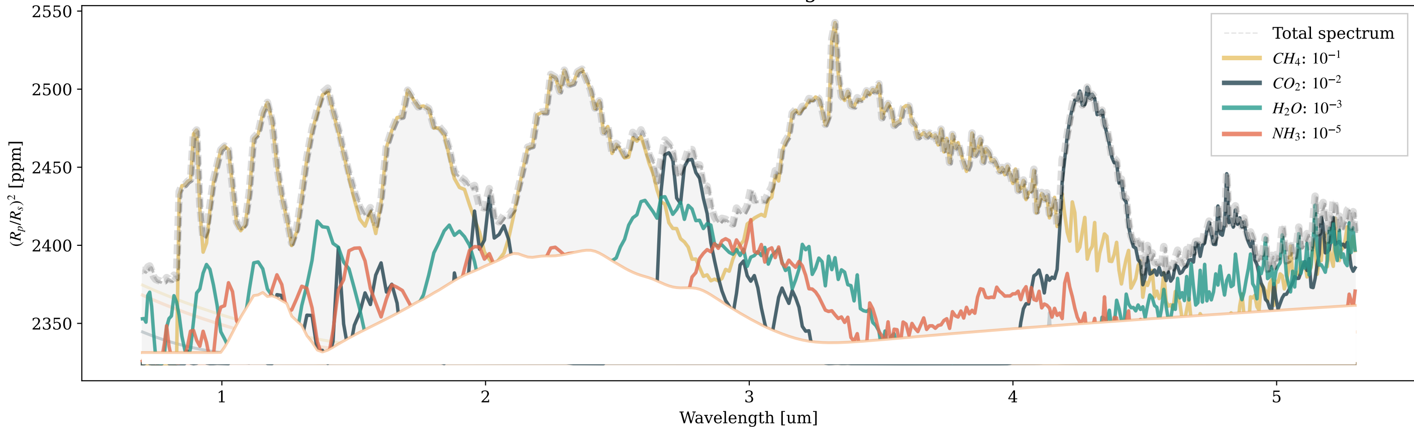
K2-18 b analogue
