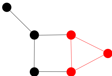
(a) Klika v grafu G_1 .
