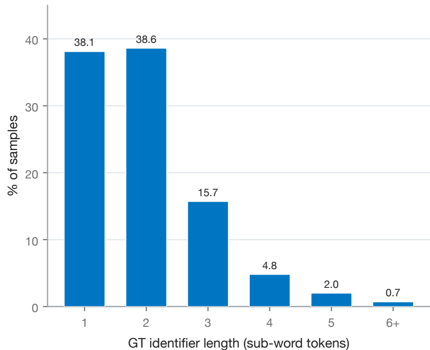
(b) GT identifier length distribution
