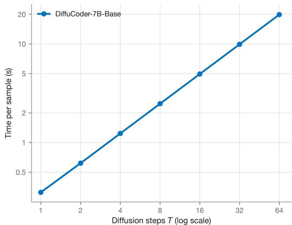
(b) Per-sample latency vs. diffusion steps
