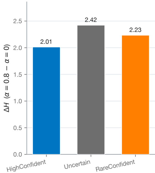
(b) Entropy increase under masking
