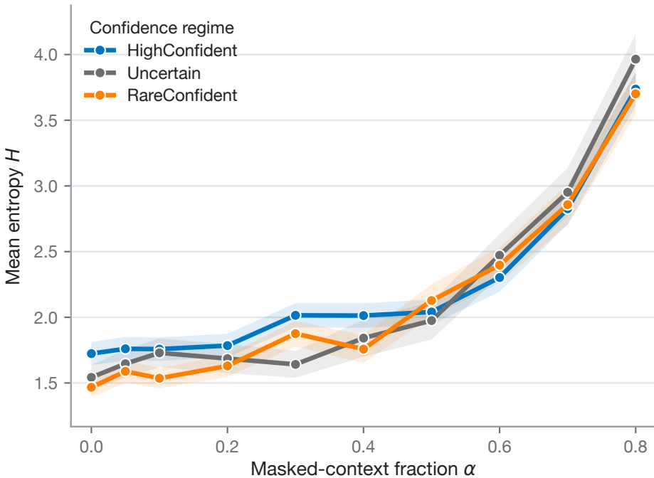
(a) Entropy vs masked-context fraction
