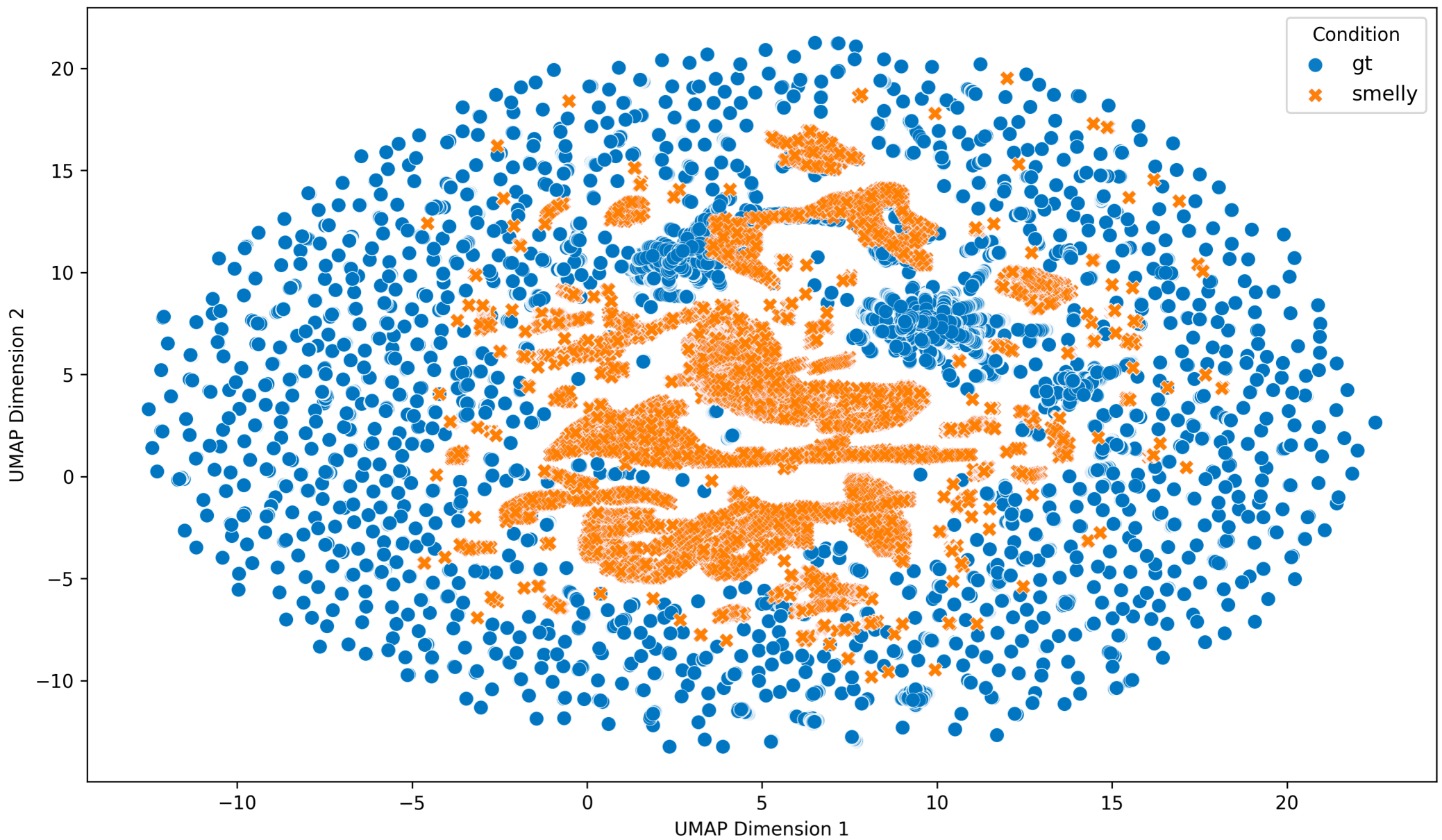
UMAP of Internal Representations — diffusion_steps (Smell Token vs. GT Token Hidden States)
