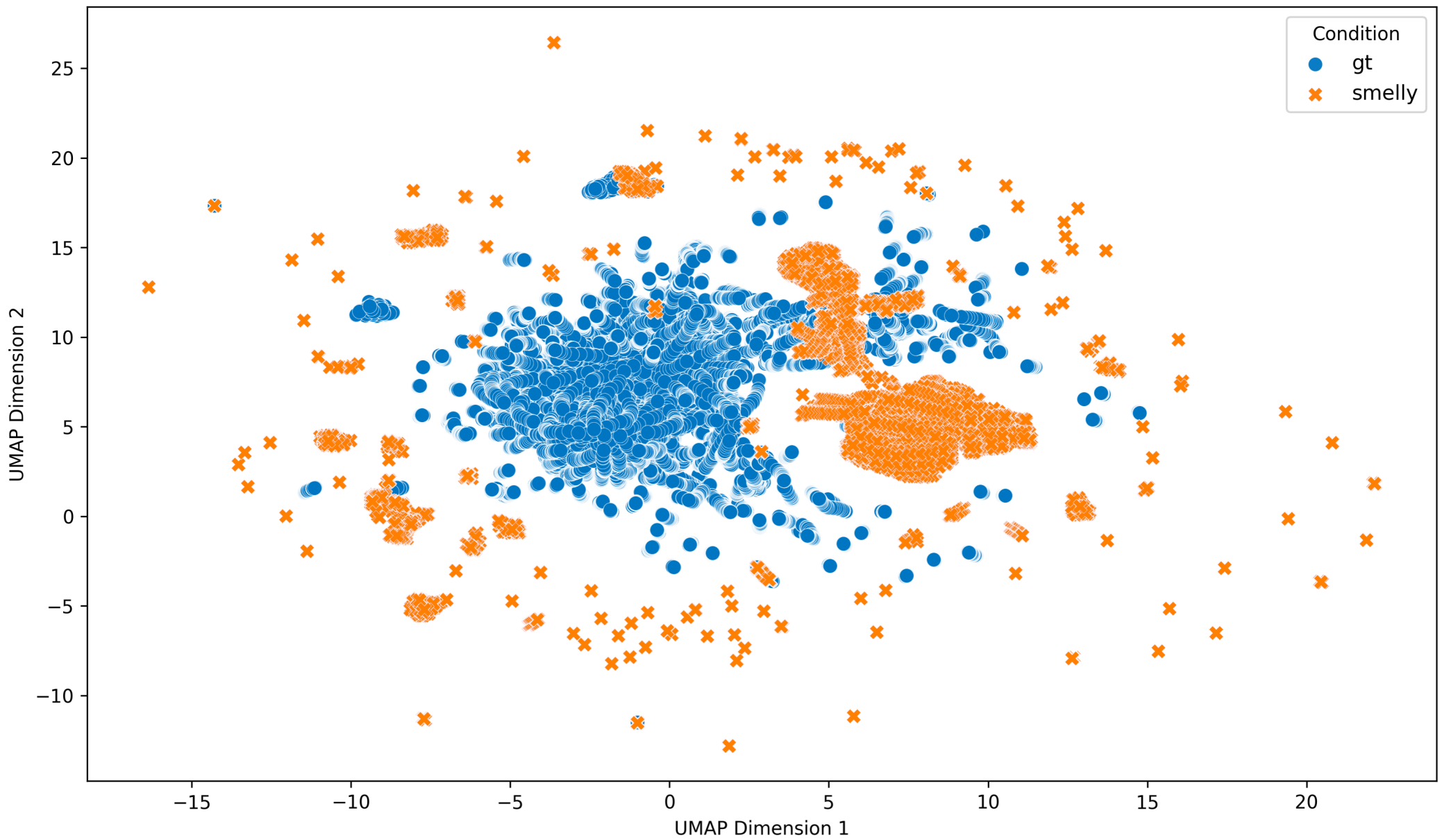
UMAP of Internal Representations — layer_wise (Smell Token vs. GT Token Hidden States)
