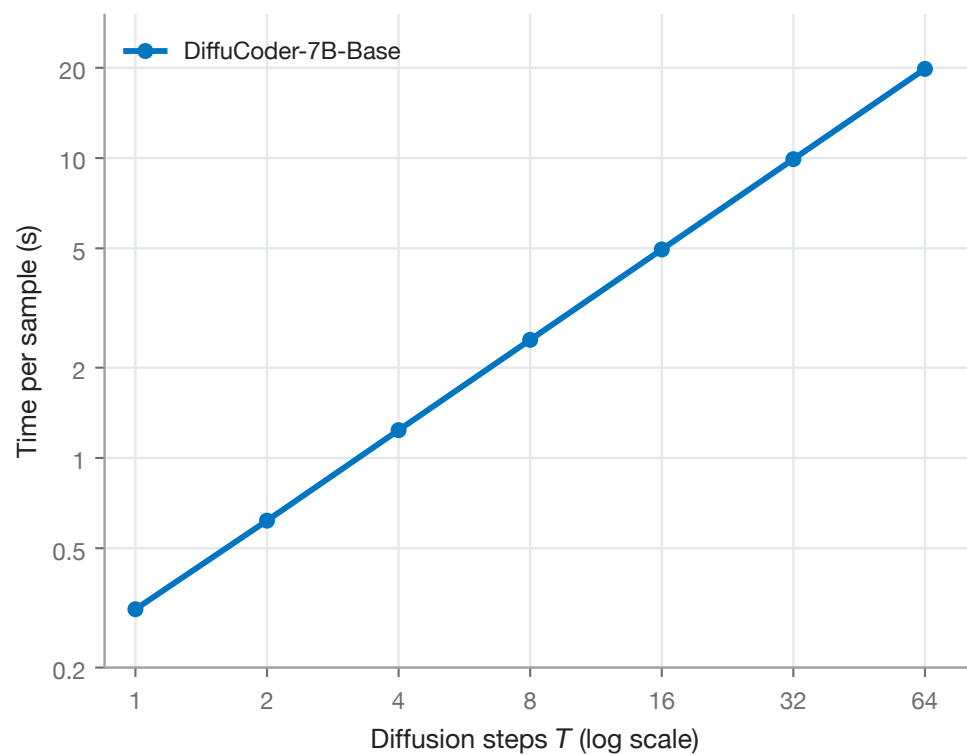
(b) Per-sample latency vs. diffusion steps
