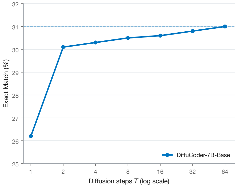
(a) Accuracy vs. diffusion steps
