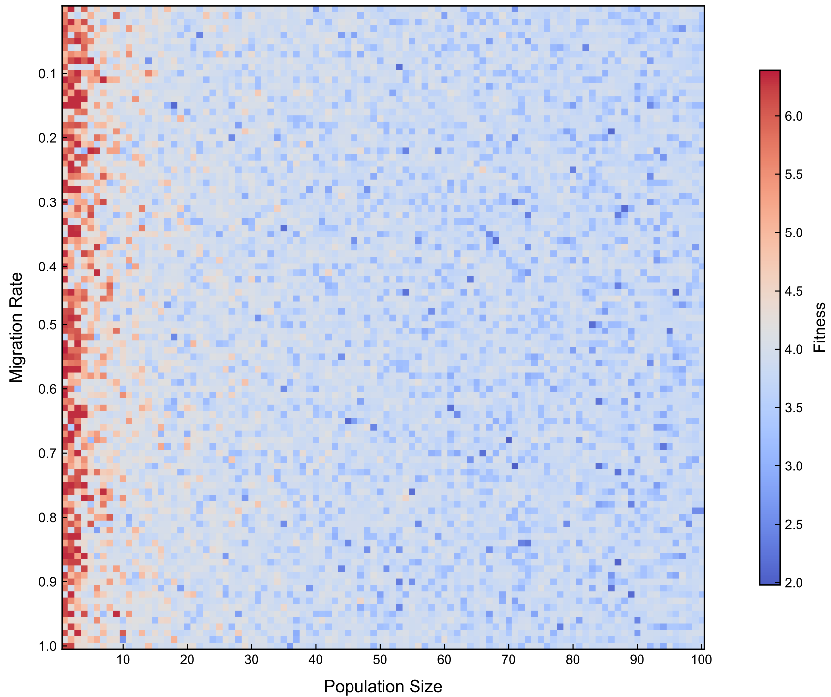
Fitness Heatmap (Neighbor Mean Fill)
