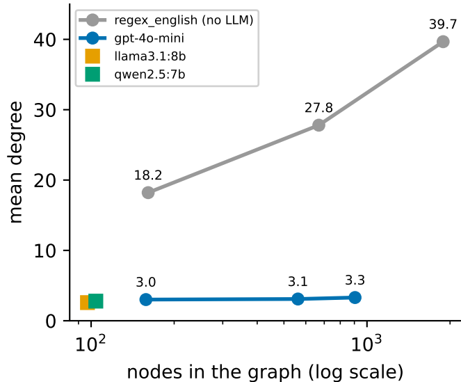
Density is set by the extraction paradigm, not by the model
