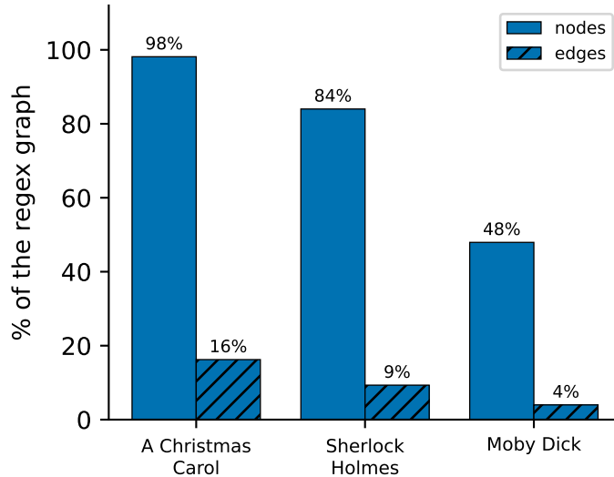
gpt-4o-mini recovers the entities, not the edges
