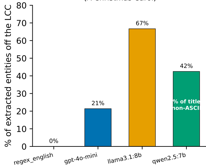
Entities the graph never connects (A Christmas Carol)
