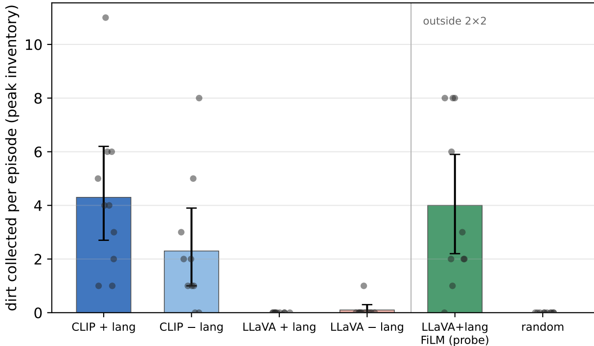
Dirt collection: CLIP digs, LLaVA anchor is a hard zero, FiLM recovers
