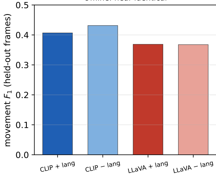
Offline: near-identical
