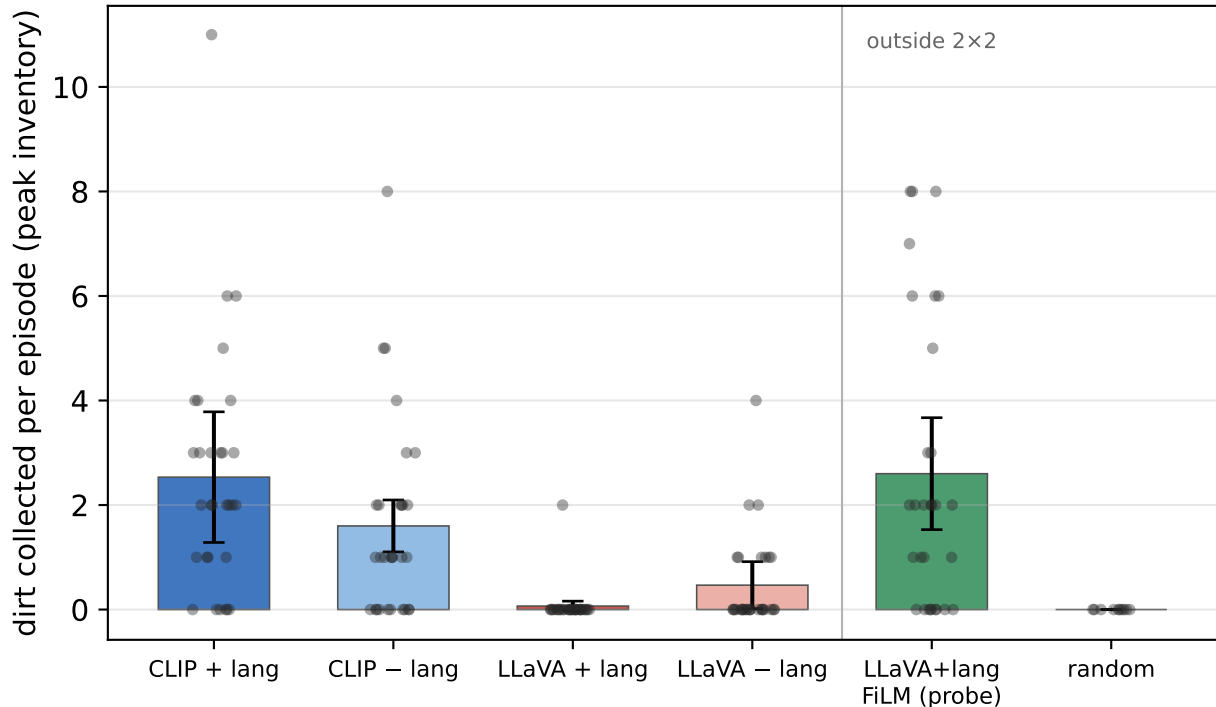
Dirt collection: CLIP digs, LLaVA anchor floors, FiLM recovers ( \approx CLIP)
