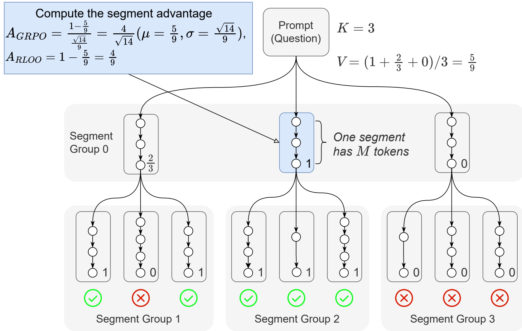
(b) Tree-Based Segment Advantage Estimation used by SPO-Tree
