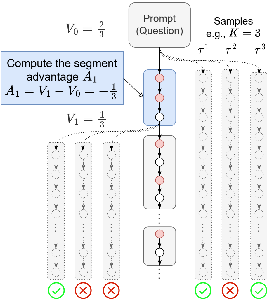
(a) Chain-Based Segment Advantage Estimation used by SPO-Chain
