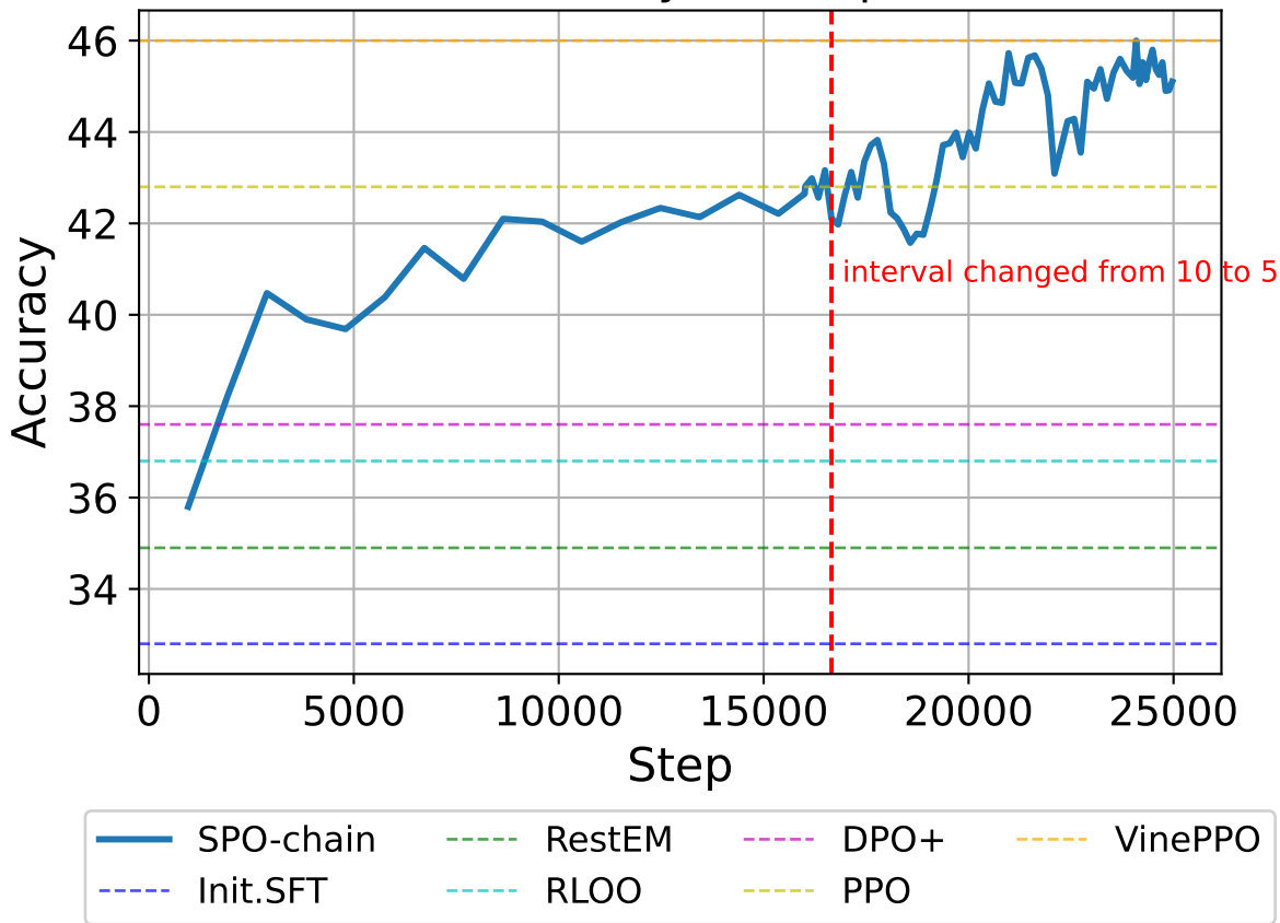
Accuracy vs. Step
