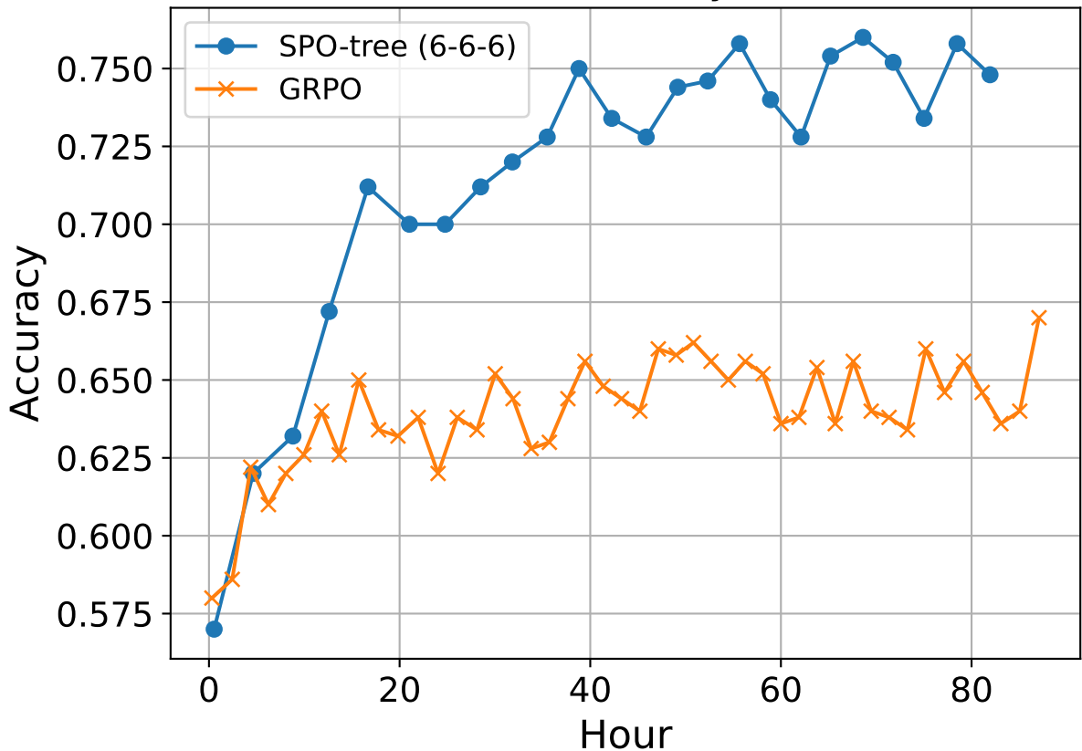
MATH500 Accuracy vs Hour
