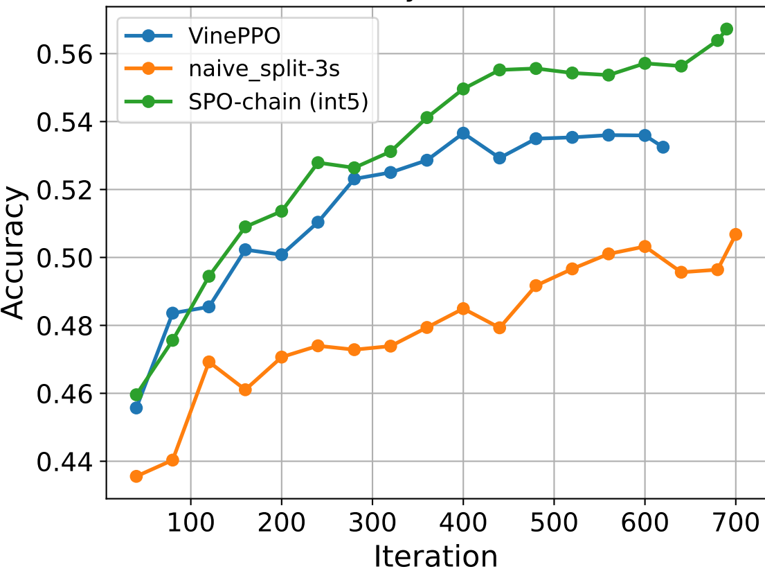
Test Accuracy Over Iterations
