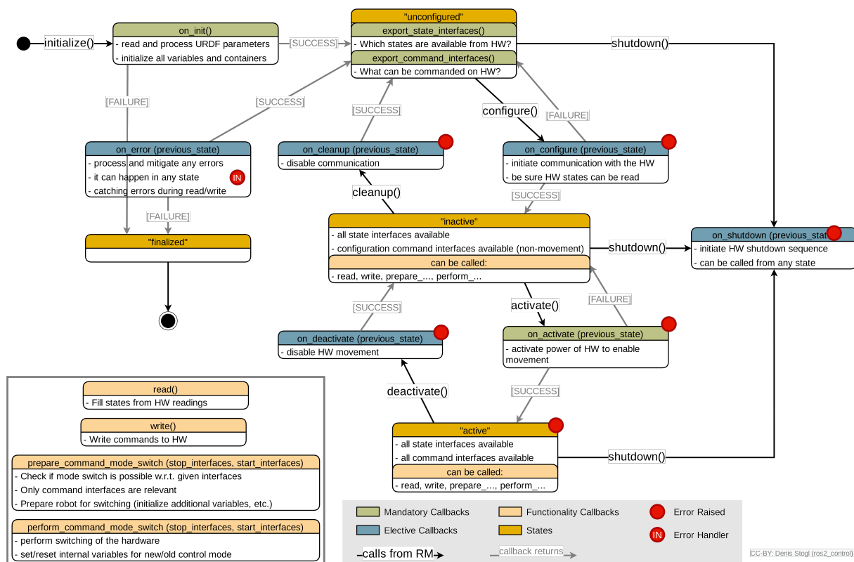
Figure 8.1 Hardware interface lifecycle
