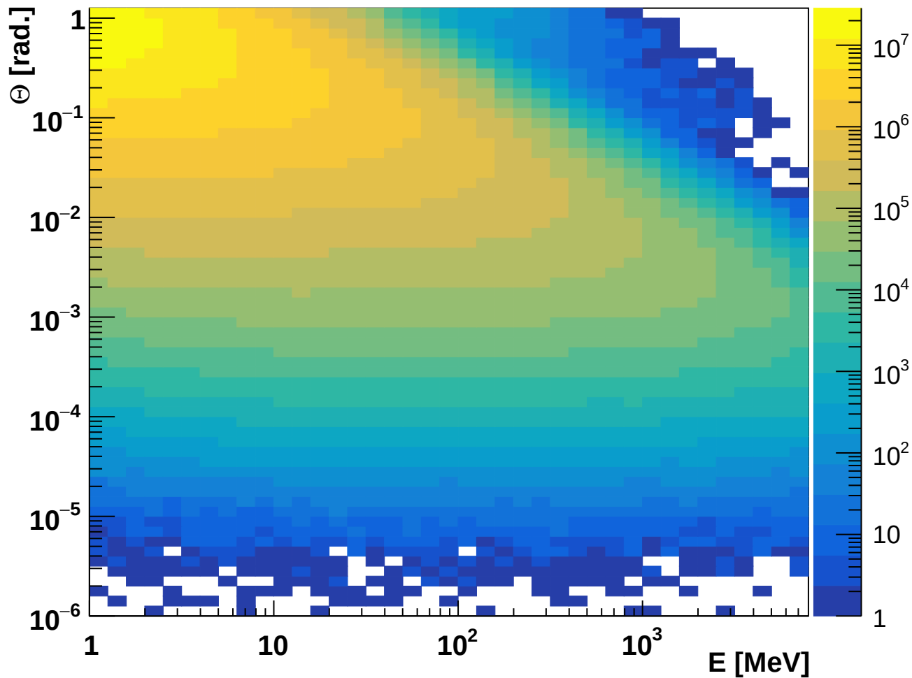
\gamma E [MeV], Theta [rad.], and Z [mm] yx projection
