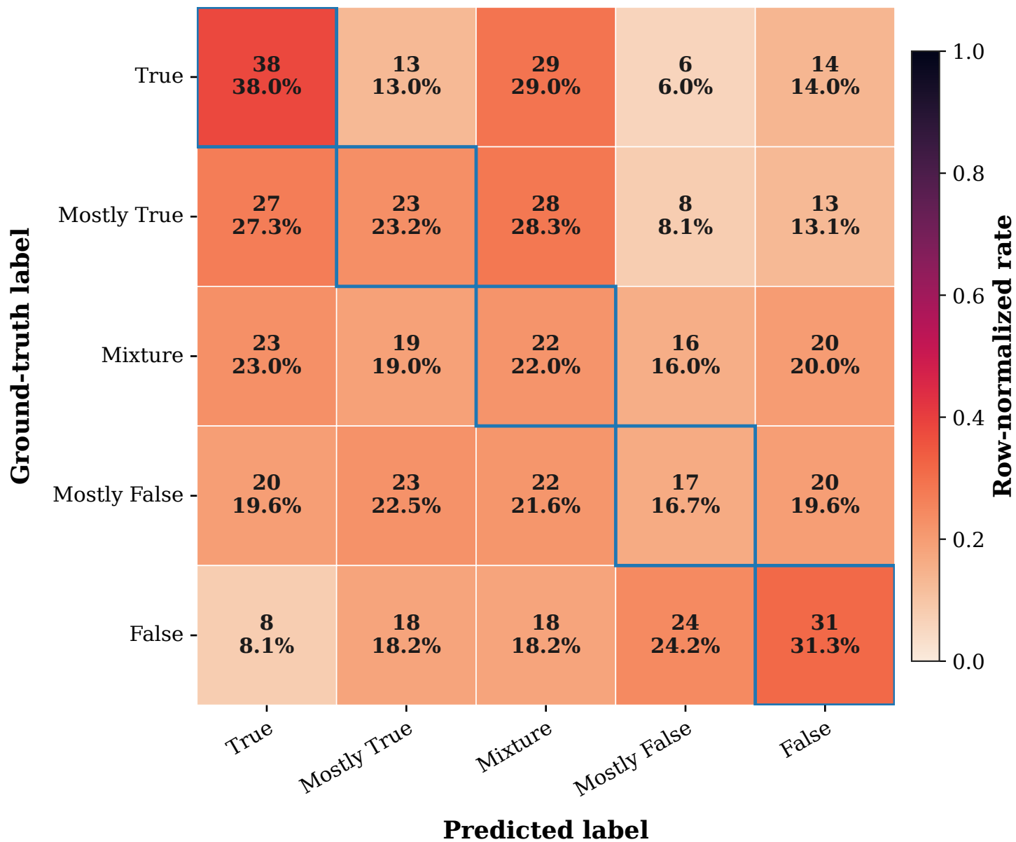
5-Class Verdict — Confusion Matrix on ReMMDBench (Model: qwen3.5-9b)
